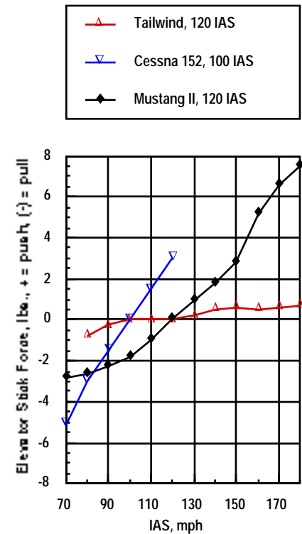
Figure 1. Static Longitudinal Stability Trimmed hands-off at V_a
