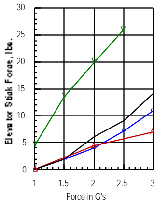
Figure 3. Maneuvering Stability @Va with mid to forward c.g.
