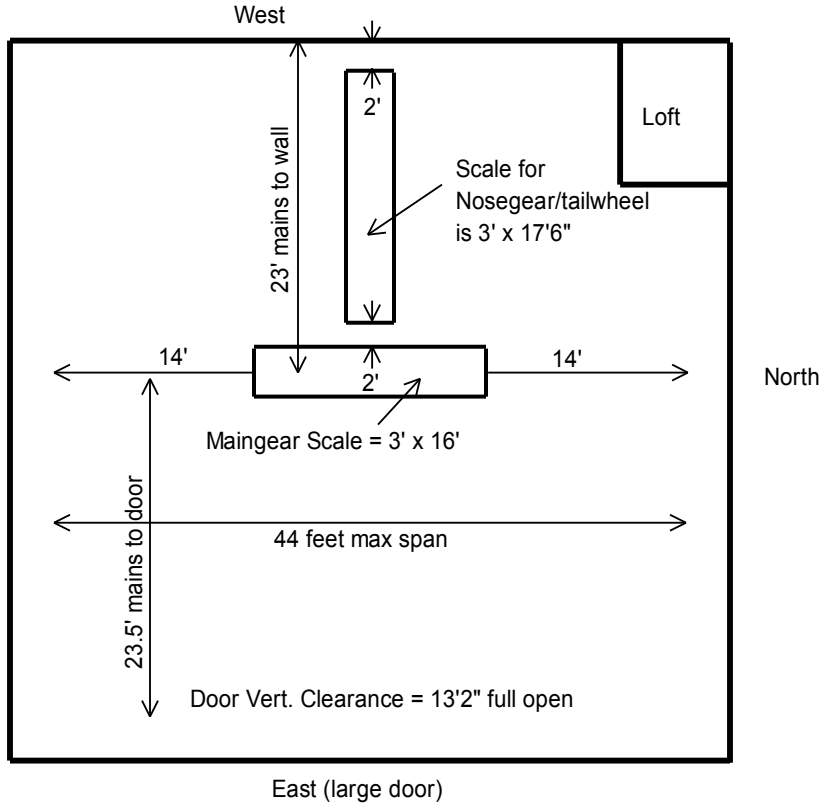
CAFE Foundation Flight Test Center Floor Plan
