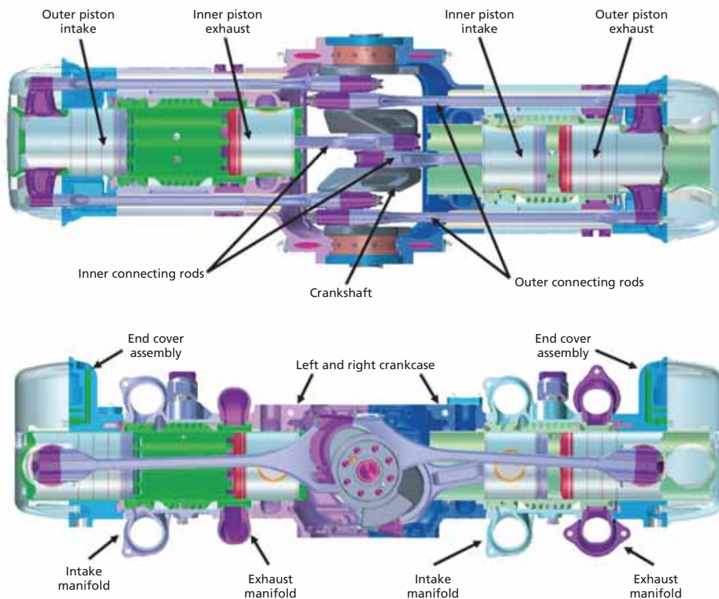
The opposed-piston, opposed-cylinder (OPOC) engine configuration being developed for military ground vehicles by FEV has all the forces acting on the crankshaft and not on the main bearings of the crankcase.
